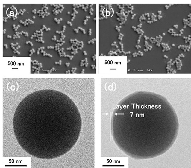
Figure 2. SEM and TEM images of PMMA nanoparticles C and PANI@PMMA core-shell nanoparticles C: a) SEM image of PMMA nanoparticles, b) SEM image of PANI@PMMA core-shell nanoparticles, c) TEM image of PMMA nanoparticles, and d) TEM image of PANI@PMMA core-shell nanoparticles.
