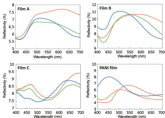
Figure 6. Reflection spectra of films A, B, C and the polyaniline film (blue: peroxidized state (pernigraniline), green: oxidized state (emeraldine salt) and red: reduced state (leucoemeraldine)).
